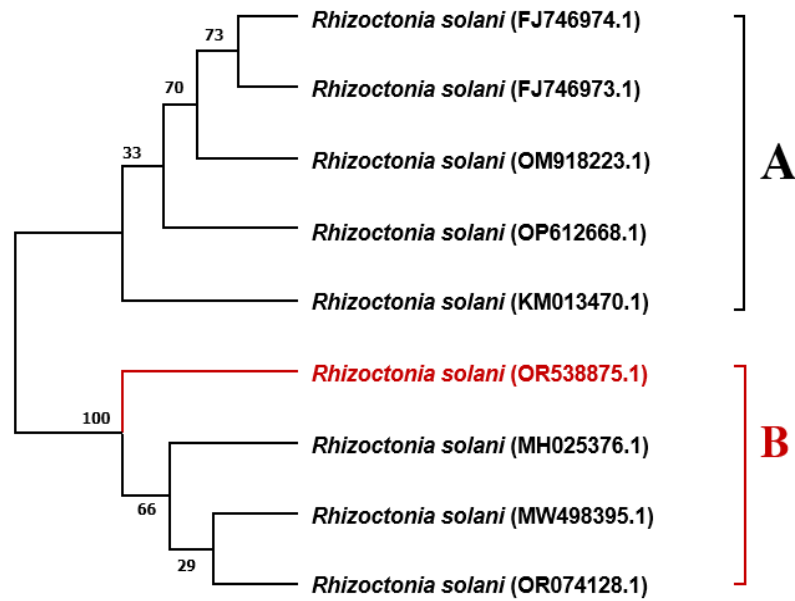
Fig.1. Phylogenetic tree based upon CLUSTAL W alignment of the ITS region of rDNA nucleotide sequences of 9 Rhizoctonia solani isolates. A maximum likelihood was used, with bootstrap values after 1000 replications of calculated run by using MEGA11 software. The branch numbers indicate bootstrap values. Our own sequenced R. solani isolate (ITS: OR538875.1). is shown in red color and the tree shows its identity with the most similar R. solani , GenBank accession numbers.
